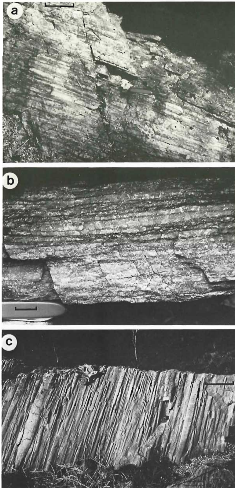
Fig. 3. Outcrop views showing markedly contrasting strain ellipsoid shapes. (a) Y - Z plane at locality 4, scale bar is 10 cm. (b) X - Z plane at locality 16, scale bar is 2 cm. (c) X - Y plane at locality 14, scale bar is 30 cm.
