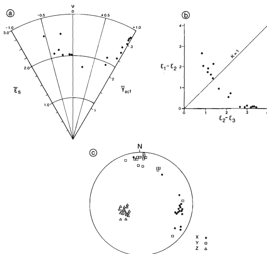
Fig. 5. Results of the strain determinations for all 17 localities. (a) Plot of the strain parameter \bar{\epsilon}_s vs Lode's parameter, \nu (see Hossack 1968). Also shown are values of \bar{\gamma}_{oct} , the natural octahedral unit shear (Nadai 1963). (b) Logarithmic deformation plot (Ramsay 1967) of same data as (a). The line labelled K = 1 is the locus of plane strain at constant volume. (c) Orientations of the principal axes of strain from the 17 locations shown on a Schmidt net.
